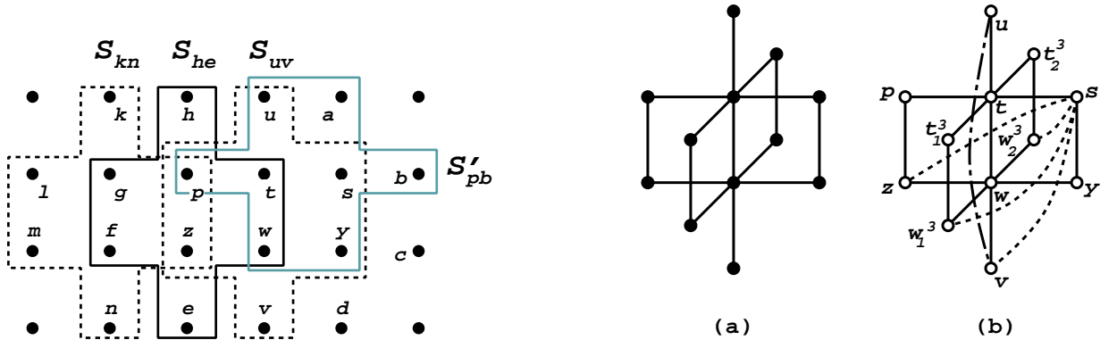
Figure 1: A plane in \mathcal{G}(\mathbb{Z}^d) , (a) Induced subgraph M in \mathcal{G}(\mathbb{Z}^3) , and (b) Dummy edges in M
