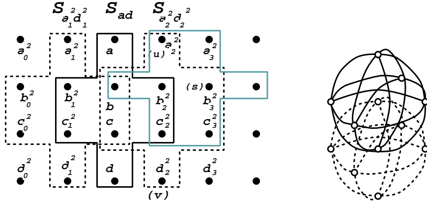
Figure 2: New nomenclature for vertices in Figure 1, and \overline{M} in \mathcal{G}(\mathbf{Z}^3) .
