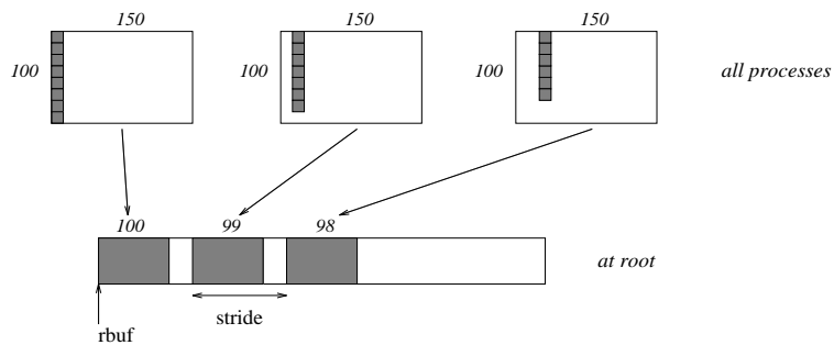
Figure 4.5 The root process gathers 100-i ints from column i of a 100 \times 150 C array, and each set is placed \text{stride} ints apart.
